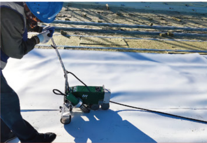
快速高效焊接TPO卷材 LST-WP1
